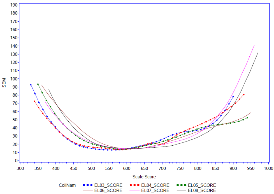
Figure 6-2 English Language Arts Standard Error Curves
